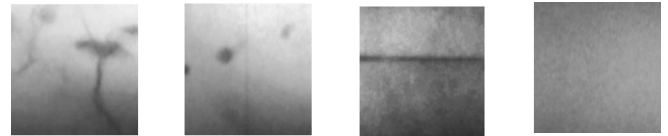
Fig. 2. Samples of 224×224 scaled tiles containing weld defects.
