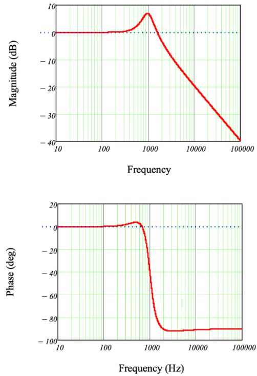
Fig. 1. G(s) Bode diagram: Magnitude (above) and phase (below).
