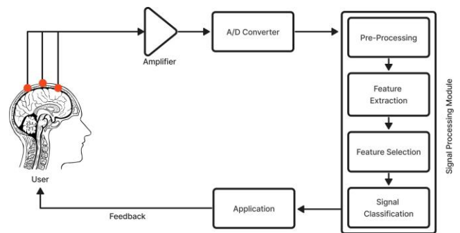
Fig.2. BCI system architecture.
