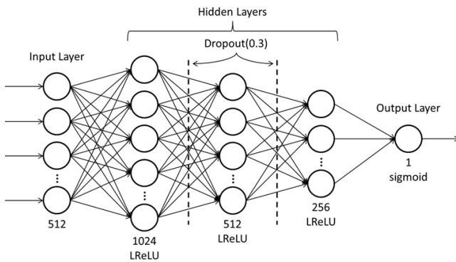
Fig. 5. Discriminator architecture.
