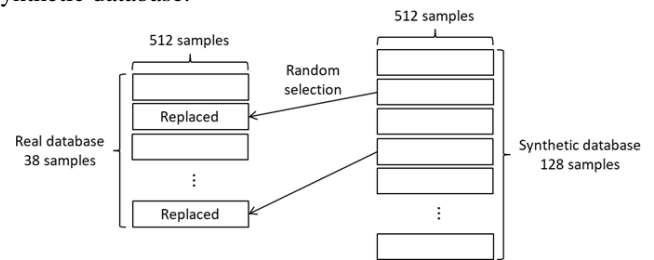
Fig. 6. Process of blending real and synthetic data.
