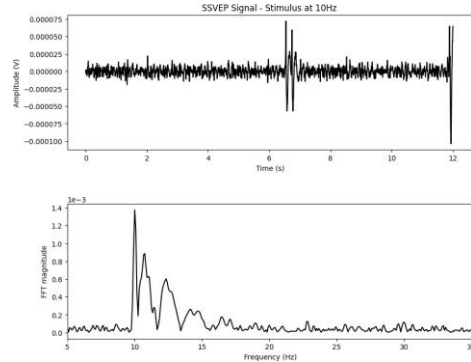
Fig.1. SSVEP signal from channel Oz in time and frequency domain.
