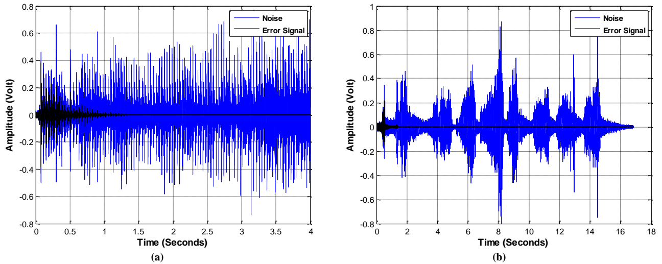
Fig. 7. Implementation of RLS on different noise sources: (a) Jackhammer, and (b) Electric saw.
