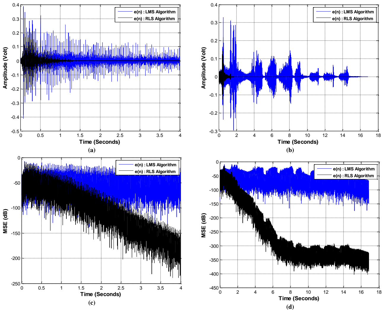
Fig. 8. Comparison of LMS and RLS algorithms implemented on different noises: (a) Jackhammer, (b) Electric saw, (c) MSE in dB for jackhammer, and (d) MSE in dB for electric saw.
