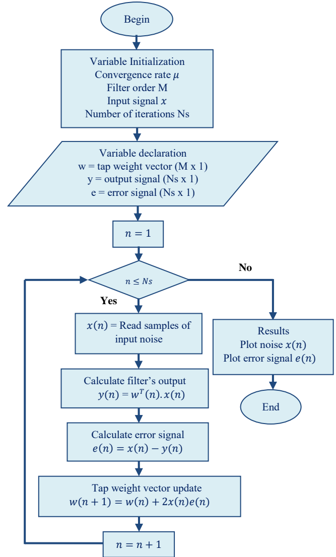
Fig. 3. Flowchart of LMS algorithm
