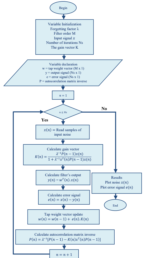
Fig. 6. Flowchart of the RLS algorithm
